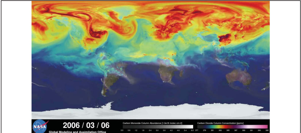
Fig. 3. \text{CO}_2 emissions and its journey in the Earth's atmosphere in winter
