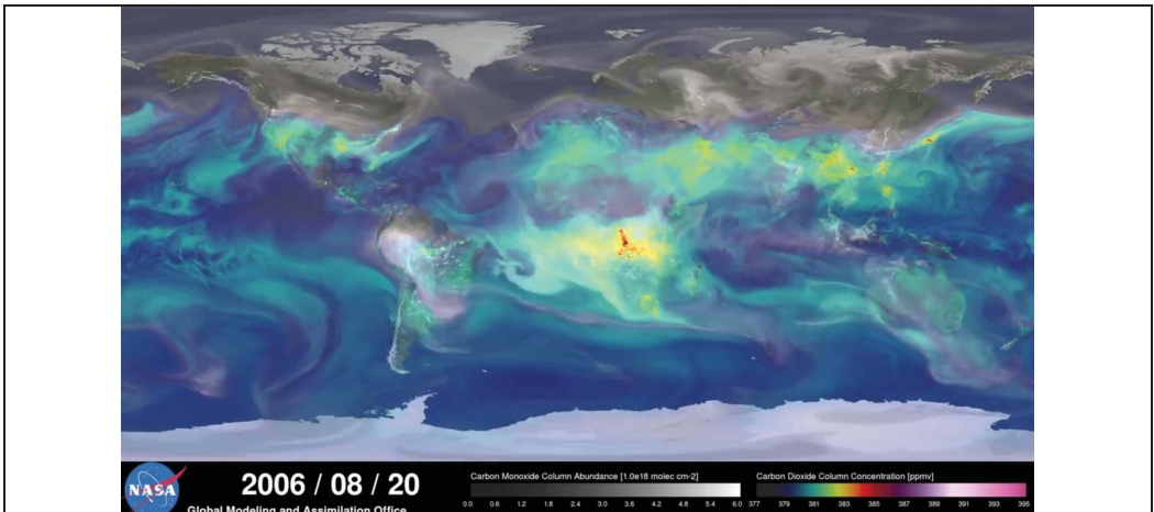
Fig. 4. \text{CO}_2 emissions and its journey in the Earth's atmosphere in summer
